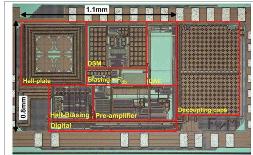
Fig. 1 Die Micrograph of the BIRD chip.
