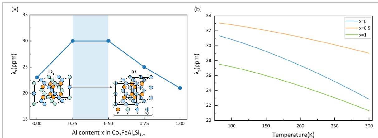
Fig. 1 (a) Room-temperature saturation magnetostriction \lambda_s versus x , showing a maximum ( \sim 30 ppm) in the intermediate compositions. (b) Temperature dependence of \lambda_s (80-300 K) with Bloch T^{3/2} fitting.
