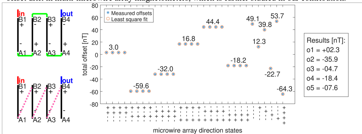
Fig. 1 Simplified microwires interconnection diagram (solid color switches can swap positions; dotted is fixed switch) and the example measurement results with sorted direction states.
