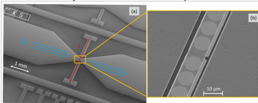
Fig. 1 (a) Scanning Electron Microscopy picture of the chip with MFCs. (b) Zoom on the MTJs below the top electrode in the MFC gap. The junctions are arranged in series-parallel blocks.
