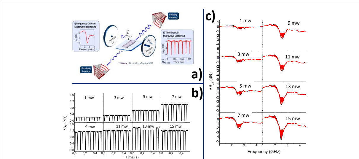
Fig. 1 a) Setup: Schematic of the microwave transmission system and Helmholtz coils ( H_{bias} ). b) Time-Domain: \Delta S_{21} evolution for an increasing number of microwires c) Frequency-Domain: \Delta S_{21} spectra showing resonance scaling with the microwire count.
