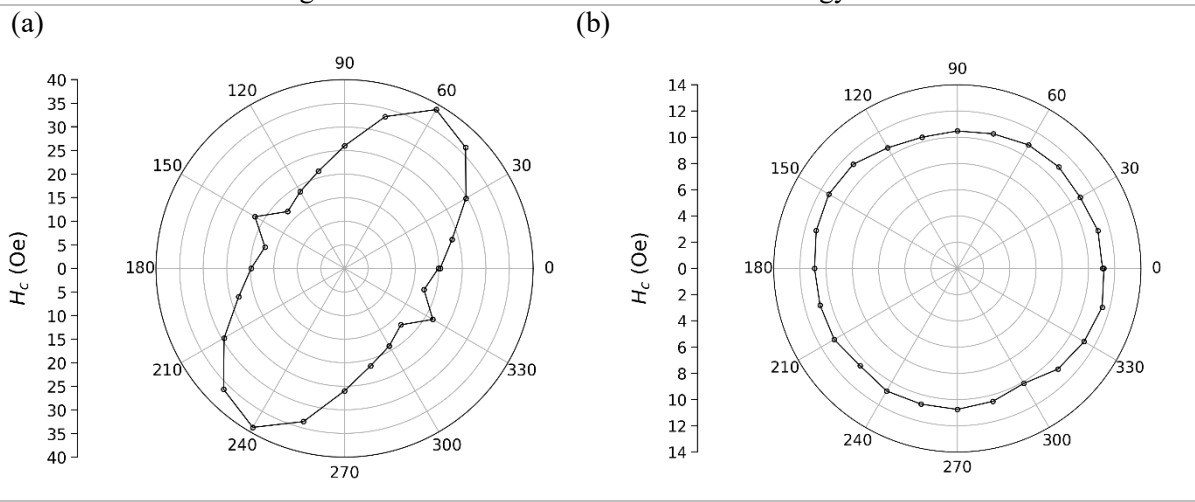
Fig. 1 Polar plots of Coercivity ( H_c ) for (a) AlScN/CoFeB/Ta (b) Si/CoFeB/Ta
