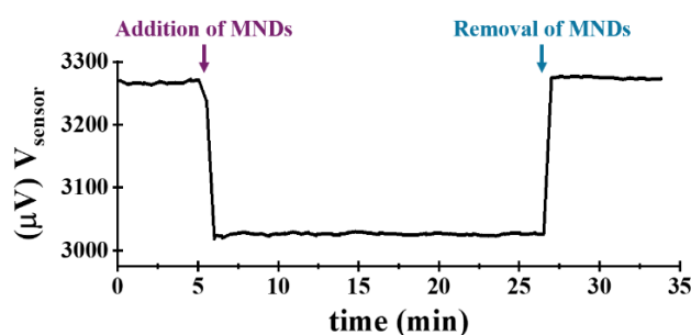
Fig. 1 Sensor voltage response upon addition and subsequent removal of MNDs.
