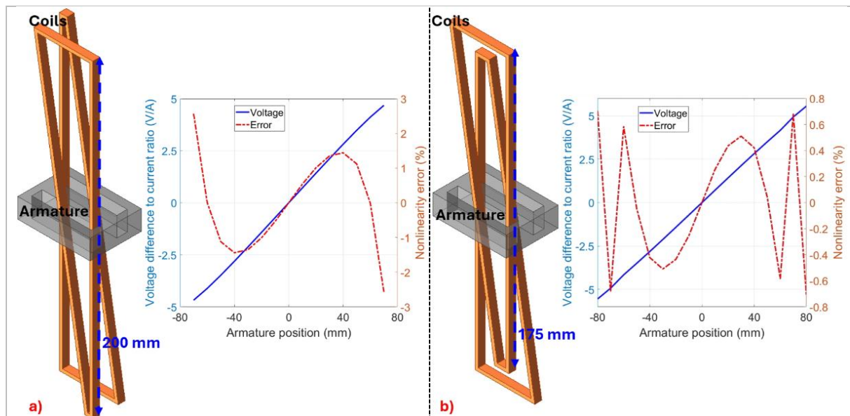
Fig. 1 The voltage difference to current ratio and nonlinearity error versus armature position, a) Initial design and b) Optimized design – Ferrite armature core
