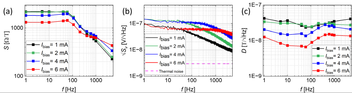
Fig. 1 Sensitivity (a), noise (b) and detectivity (c) of the skyrmion Hall sensor for different bias currents from 1 to 6 mA.
