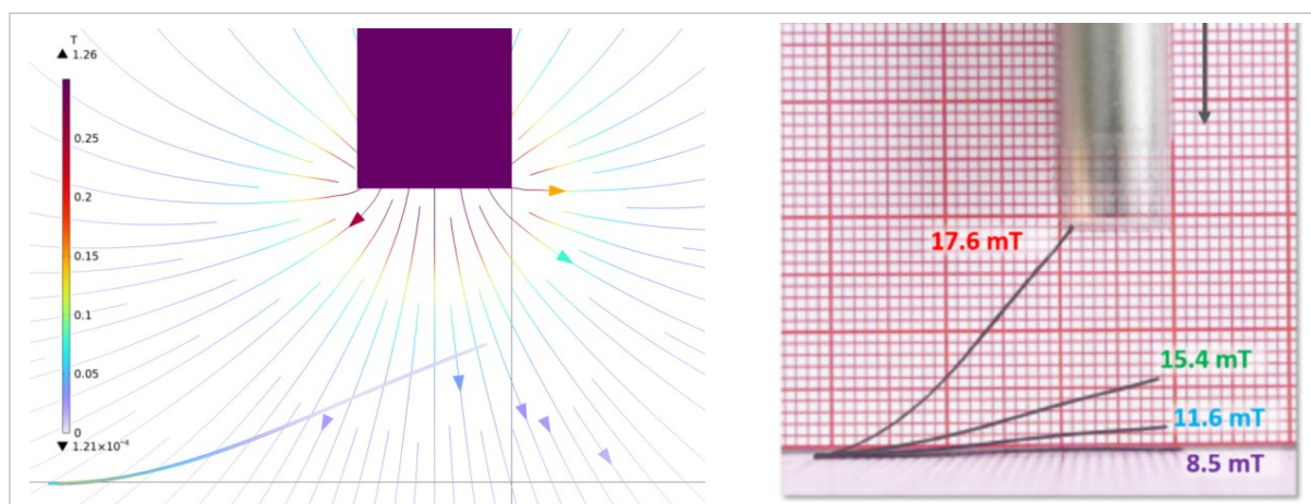
Fig. 1: Elastic deformation of the composite strip in the presence of a magnet bar: finite element simulations (left) and experimental results (right).
