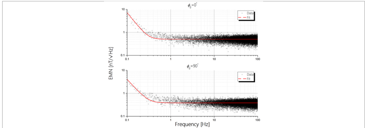
Fig. 1 EMN spectra of an EPHE sensor for two anisotropy configurations: parallel alignment (top, H_{\text{eff}} = 5.4 Oe, EMN = 50.3 pT/ \sqrt{\text{Hz/A}} at 1 Hz) and perpendicular alignment (bottom, H_{\text{eff}} = 3.8 Oe, EMN = 38.3 pT/ \sqrt{\text{Hz/A}} at 1 Hz). Markers: measured data; solid line: fit. The perpendicular configuration shows a lower noise floor due to the reduced effective anisotropy.
