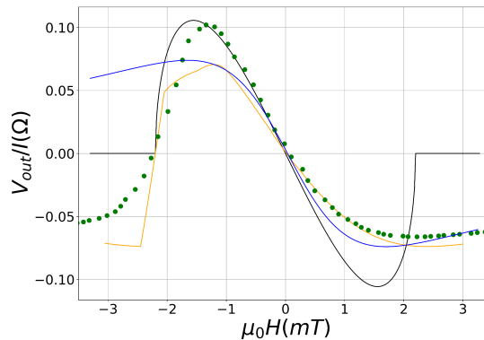
Fig. 1 Wheatstone bridge SMR sensor output (Pt/FeCoB) as a function of the applied field, at I = 5\text{mA} (green dots). Predictions from the Stoner-Wohlfarth model without (black line) and with misalignment of an angle \beta = 0.3 (orange line); prediction with the LLG model (blue line).
